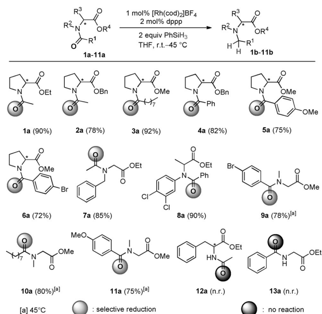
Scheme 2. Substrate scope for the selective reduction of tertiary and secondary N -acylamino acid esters. Yields of isolated products are given in parenthesis.
